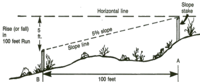
Figure 3. Image showing how slope percent is determined. Figure from Soil and the Environment: A Land and Homesite Evaluation Handbook and Training Guide . (University of Idaho - Bulletin 795)
